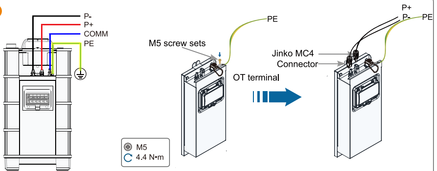
Connection Diagram
