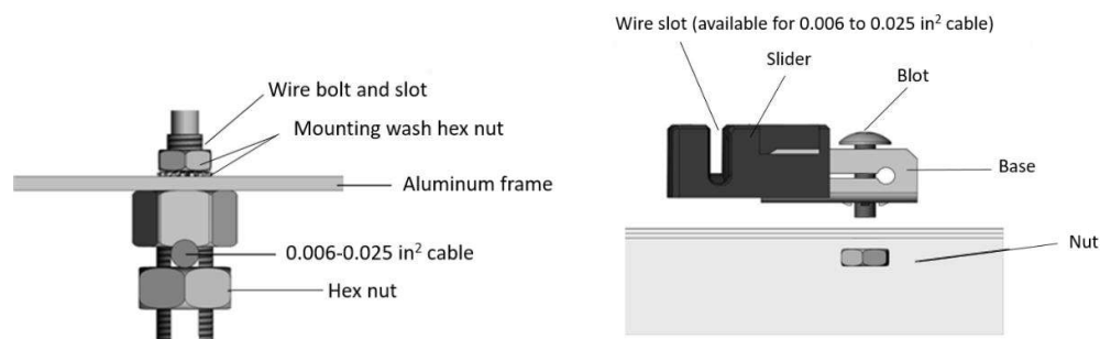
Figure 4. PV module grounding methods (IEC standard).
