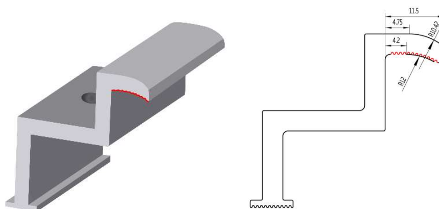
Figure 3. A surface matching clamp
