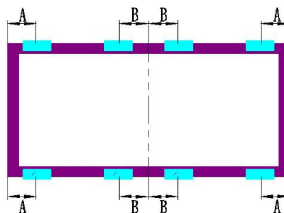
Use 8 clamps on the long side.
