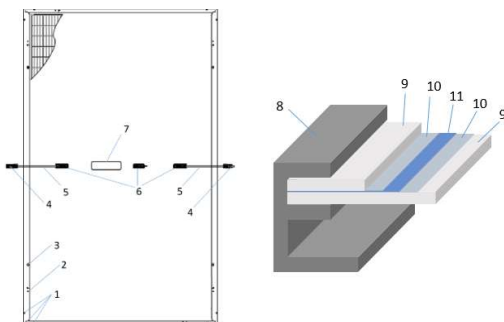
Mechanical drawing for bifacial modules
