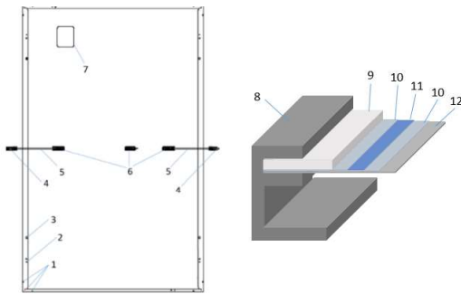
Mechanical drawing for monofacial modules
