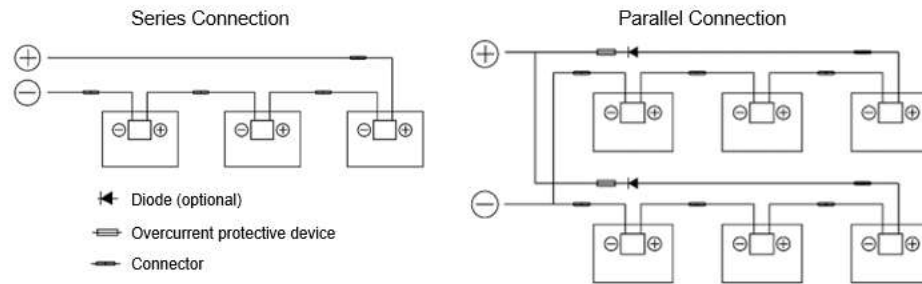
Figure 6. Series and parallel connection circuit diagram.
